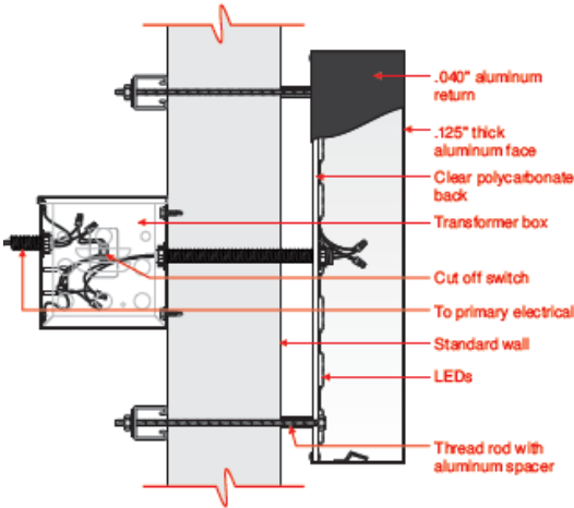
Typical Halo Illuminated LED Channel Letter Detail NTS
