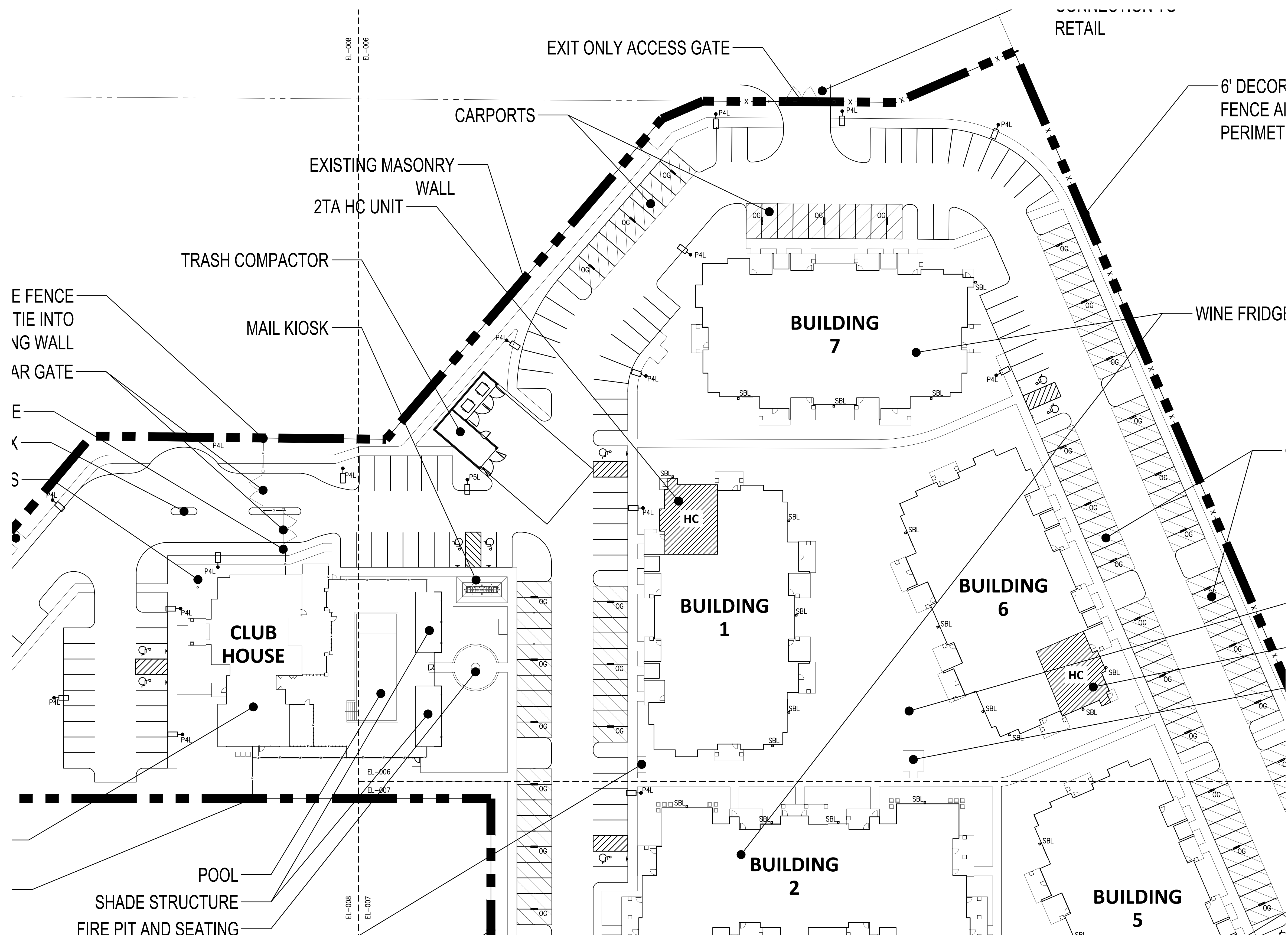
1 SITE LIGHTING - FIXTURE LOCATIONS 1" = 60'-0"
