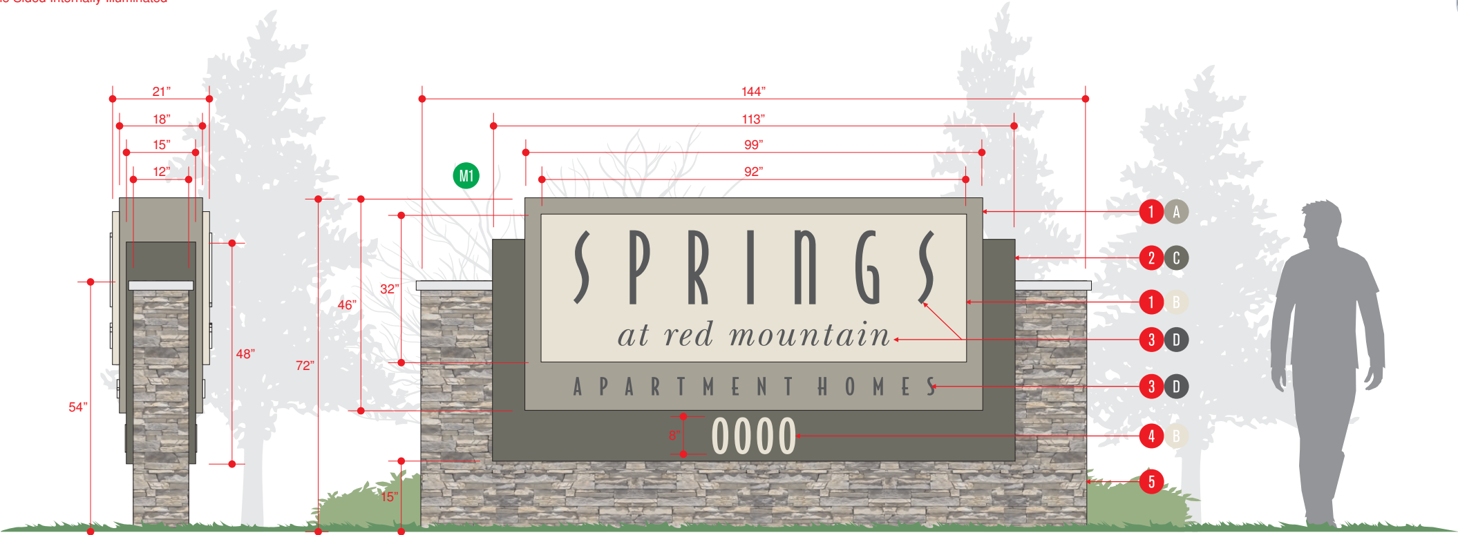
Side View
